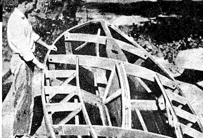
In addition to the deck framing—the mast step, mast partner, and the centerboard well are fastened in place.
