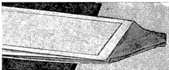
Canvas encloses the transom end of the boat. It is stretched tight when the plywood transom and transom seat are in place.
