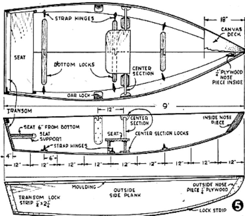
The completed boat with a canvas "deck" stretched across the bow. Removable center section with seat, the plywood transom, and the transom seat hold the boat rigid when it is opened up. The parts named can be taken out or installed quickly.
