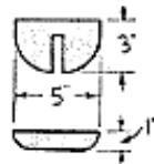
CENTER SECTION LOCK PIECES \frac{3}{8} " PLYWOOD (2 - 3'x5" AND 4 - 1'x5" PIECES NEEDED)
