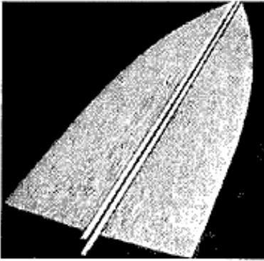
The two bottom pieces are joined along the keel line with a strip of canvas locked in place with two wooden strips. Marine glue makes it tight.
