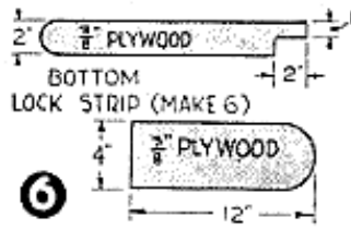
OAR LOCK BLOCK (MAKE 2)
